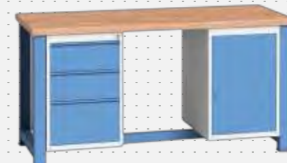
MEDIUM BENCH KA/41700A/1x3ZV/1xSV 840/1700/700 - V-Š-H Pracovná doska – 40 mm
